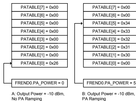
Figure 24: PA Ramping
